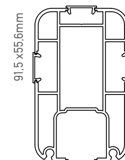
BRIDGE - SKY Profile
